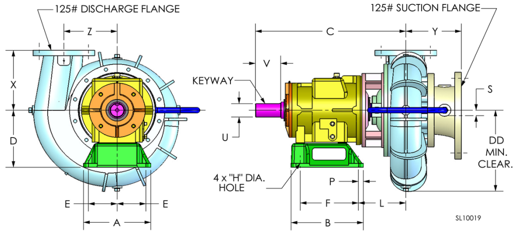
PUMP DIMENSIONS
